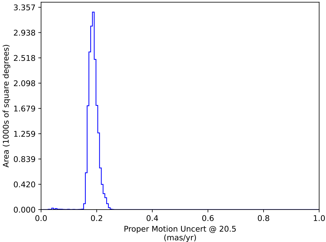
mw_roll_all_v3.3_10yrs WFD: Proper Motion Uncert @ 20.5
