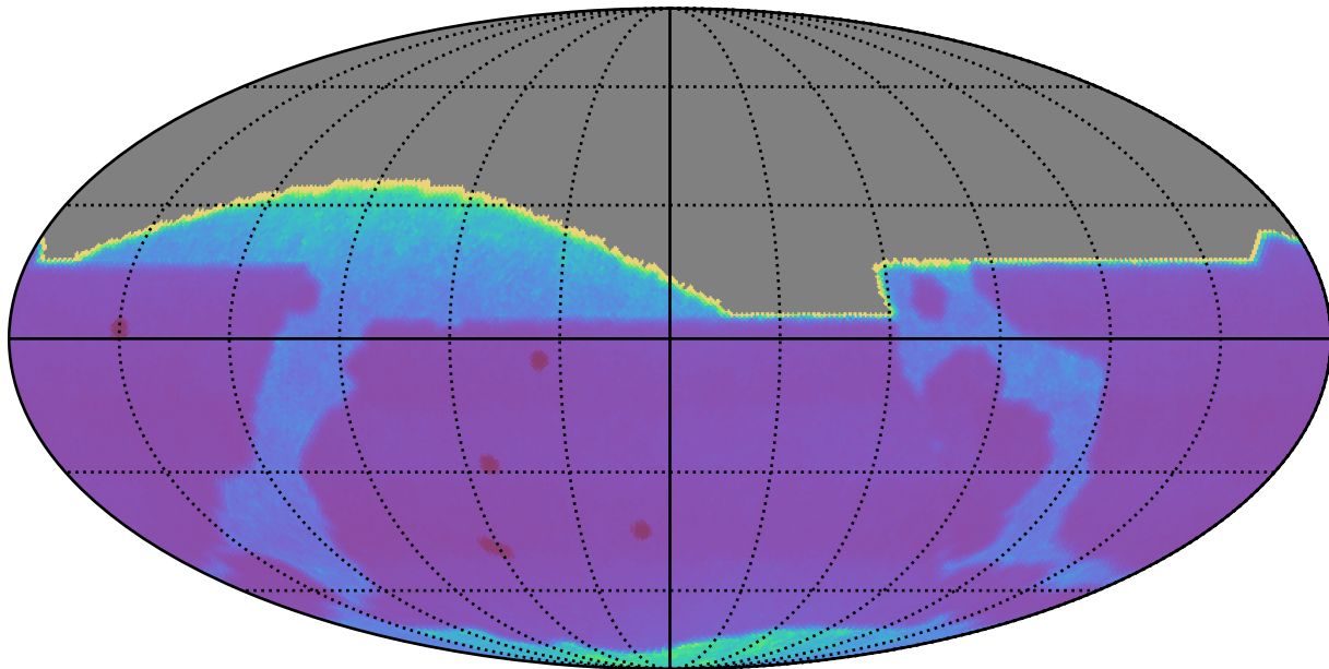
mw_roll_all_v3.3_10yrs All sky: Proper Motion Uncert @ 20.5
