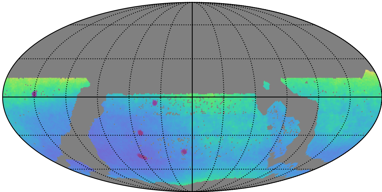
mw_roll_all_v3.3_10yrs WFD: Parallax Uncert @ 24.0
