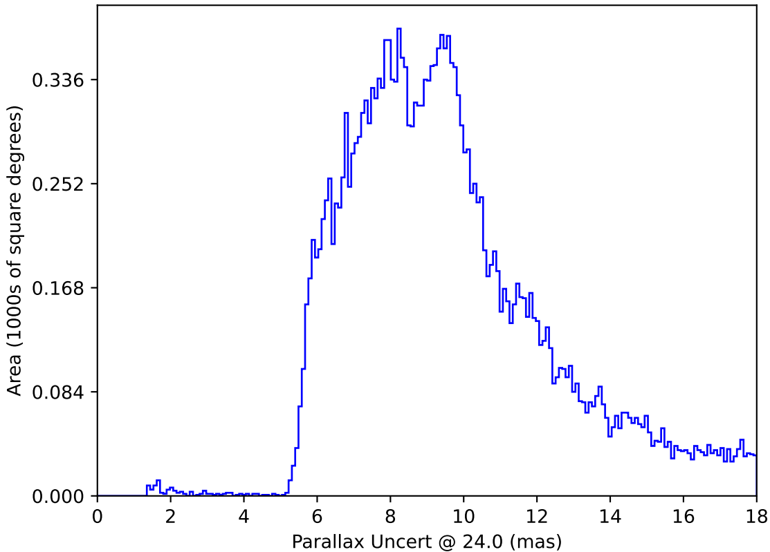
mw_roll_all_v3.3_10yrs All sky: Parallax Uncert @ 24.0
