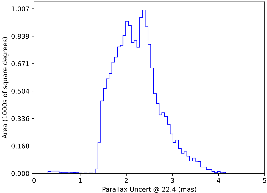
mw_roll_all_v3.3_10yrs WFD: Parallax Uncert @ 22.4
