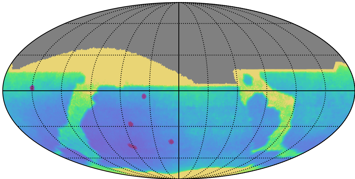
mw_roll_all_v3.3_10yrs All sky: Parallax Uncert @ 22.4
