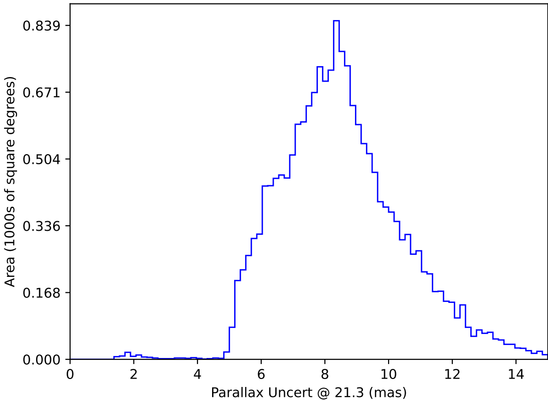
mw_roll_all_v3.3_10yrs WFD y band only: Parallax Uncert @ 21.3
