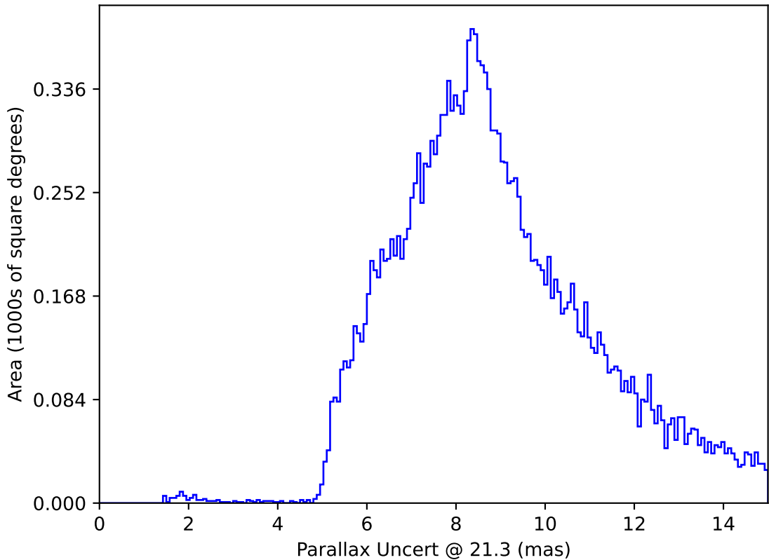
mw_roll_all_v3.3_10yrs All sky y band only: Parallax Uncert @ 21.3
