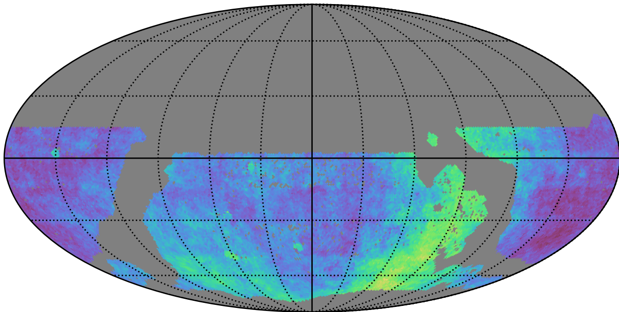
mw_roll_all_v3.3_10yrs WFD: Parallax Coverage @ 24.0
