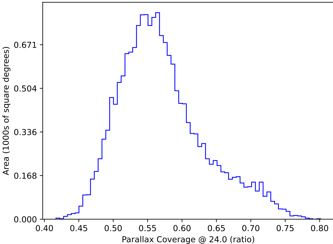
mw_roll_all_v3.3_10yrs WFD: Parallax Coverage @ 24.0
