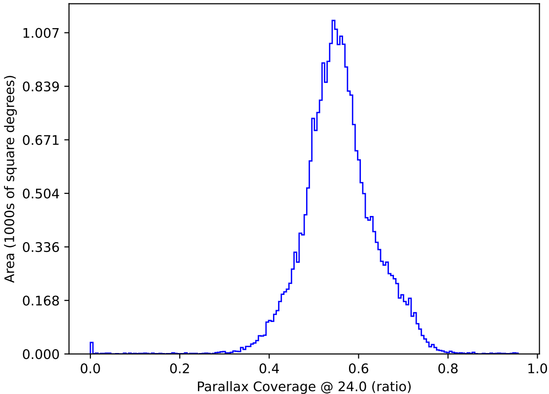
mw_roll_all_v3.3_10yrs All sky: Parallax Coverage @ 24.0
