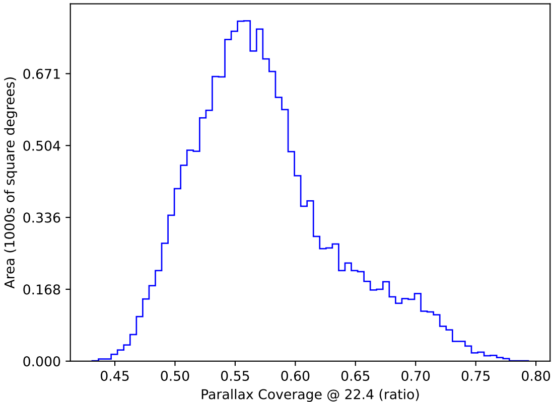
mw_roll_all_v3.3_10yrs WFD: Parallax Coverage @ 22.4
