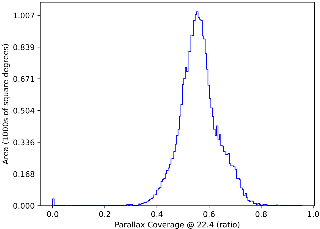
mw_roll_all_v3.3_10yrs All sky: Parallax Coverage @ 22.4
