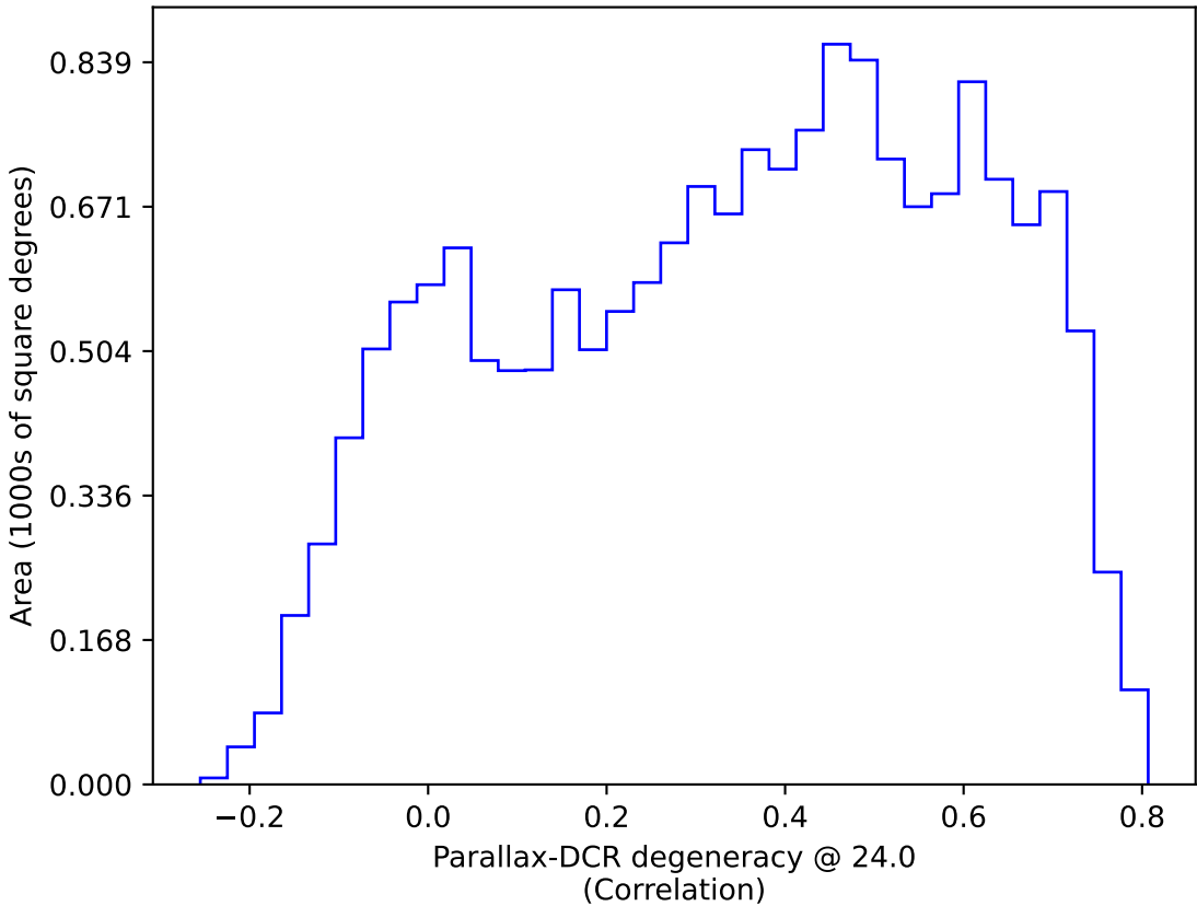
mw_roll_all_v3.3_10yrs WFD: Parallax-DCR degeneracy @ 24.0
