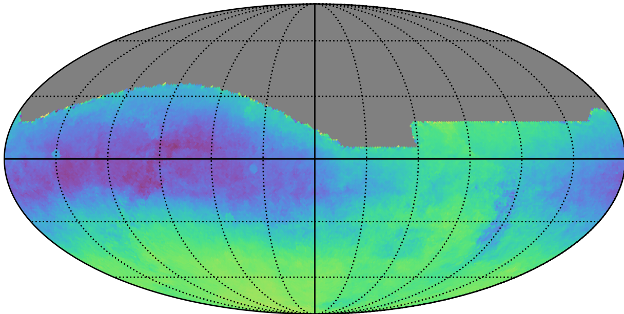
mw_roll_all_v3.3_10yrs All sky: Parallax-DCR degeneracy @ 24.0
