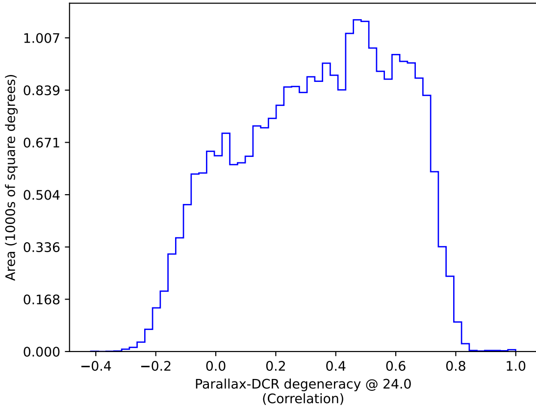
mw_roll_all_v3.3_10yrs All sky: Parallax-DCR degeneracy @ 24.0
