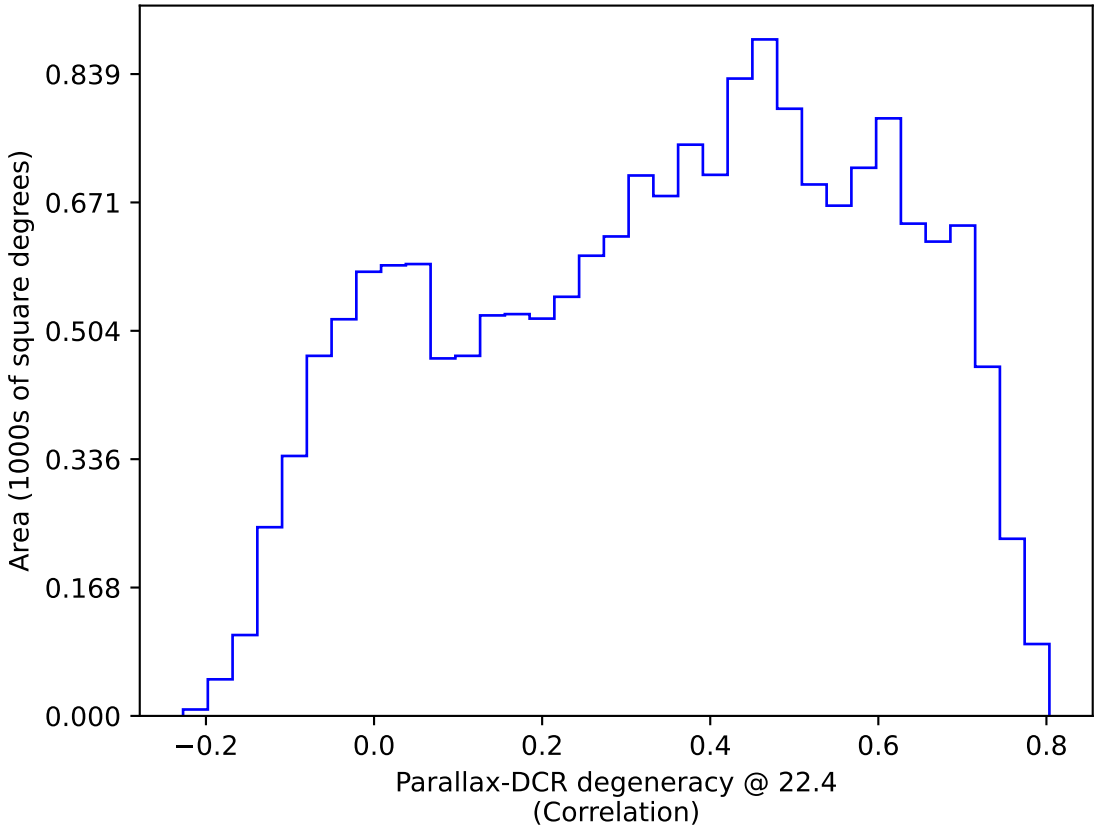
mw_roll_all_v3.3_10yrs WFD: Parallax-DCR degeneracy @ 22.4
