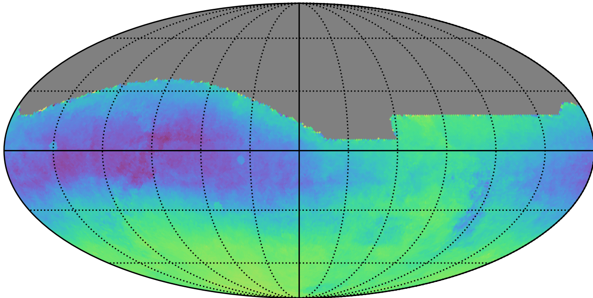
mw_roll_all_v3.3_10yrs All sky: Parallax-DCR degeneracy @ 22.4
