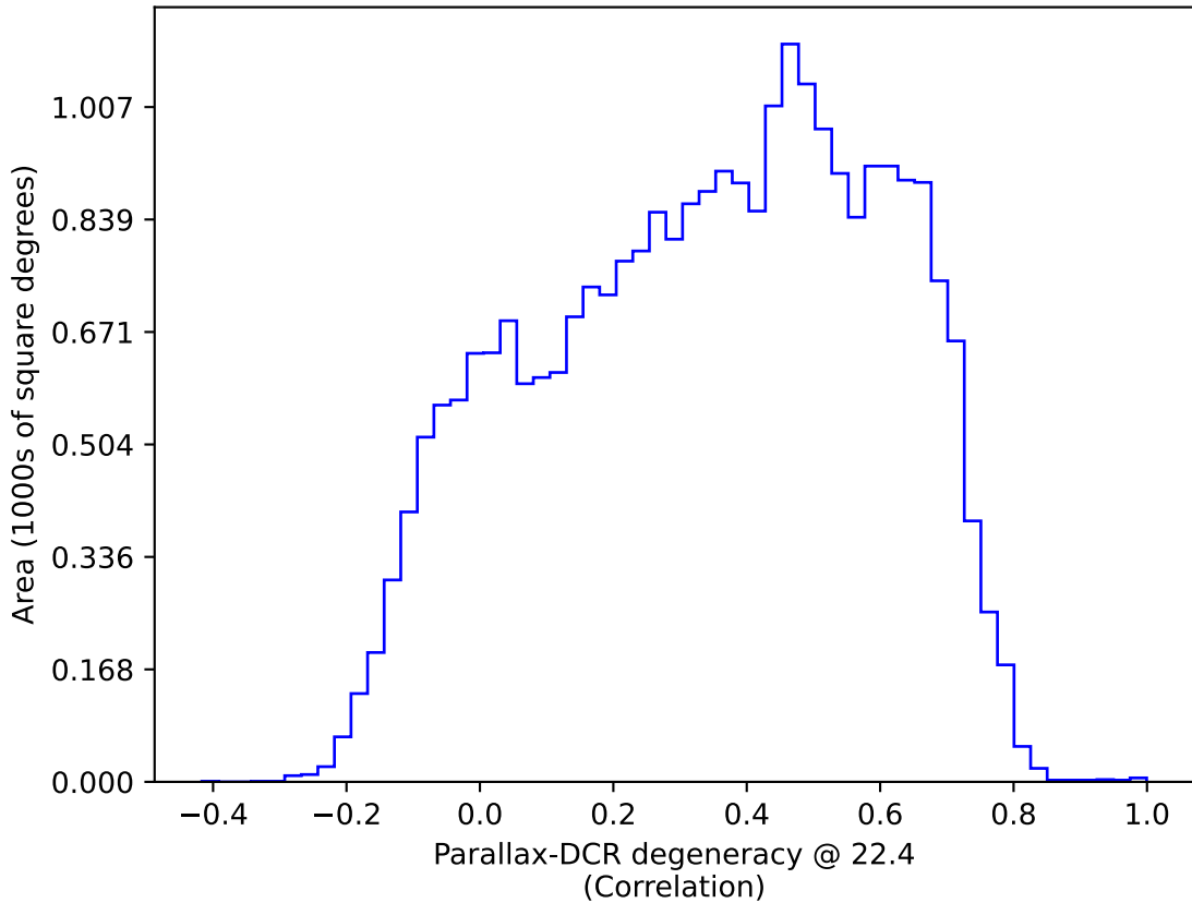
mw_roll_all_v3.3_10yrs All sky: Parallax-DCR degeneracy @ 22.4
