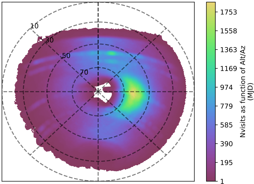
mw_roll_all_v3.3_10yrs y band: Nvisits as function of Alt/Az
