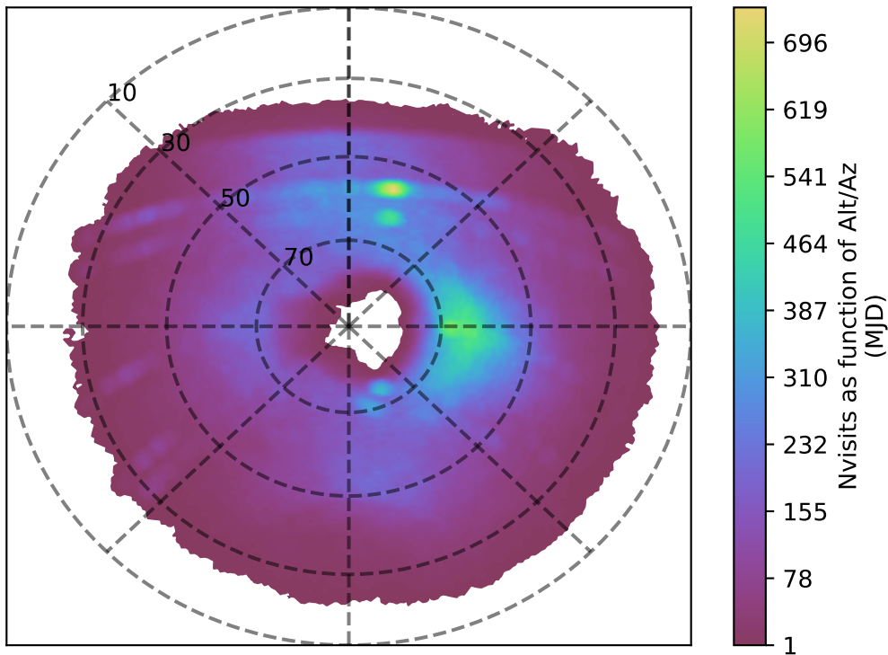
mw_roll_all_v3.3_10yrs u band: Nvisits as function of Alt/Az
