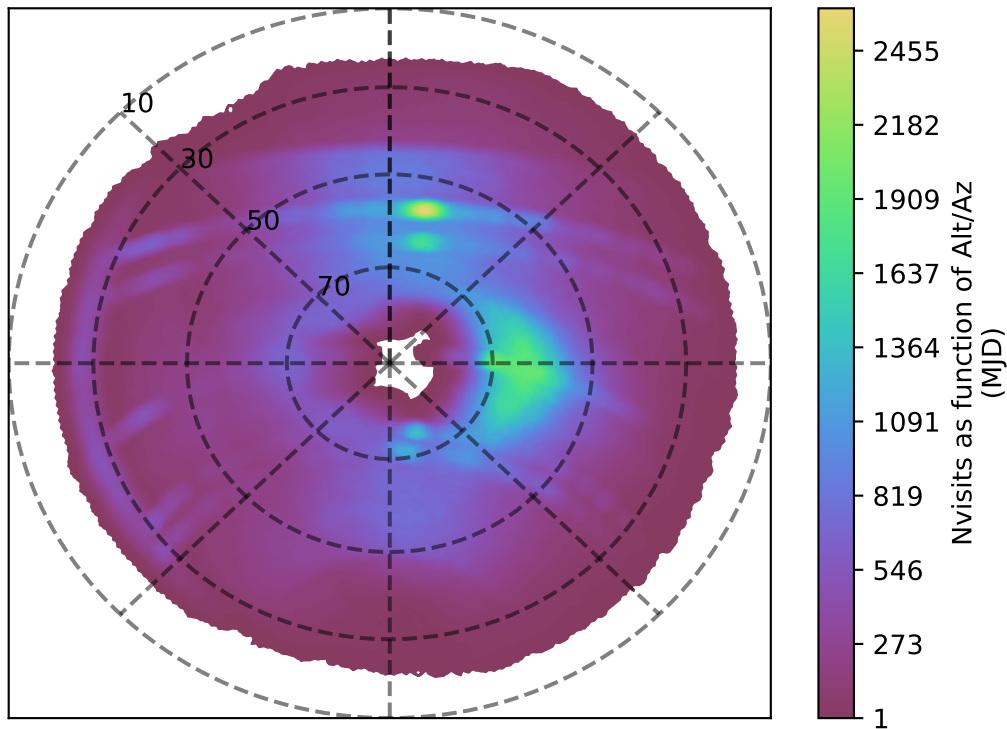
mw_roll_all_v3.3_10yrs r band: Nvisits as function of Alt/Az
