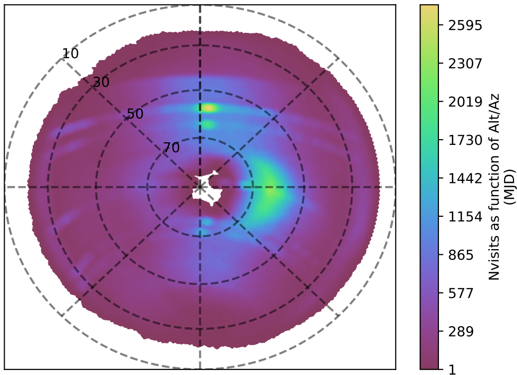
mw_roll_all_v3.3_10yrs i band: Nvisits as function of Alt/Az
