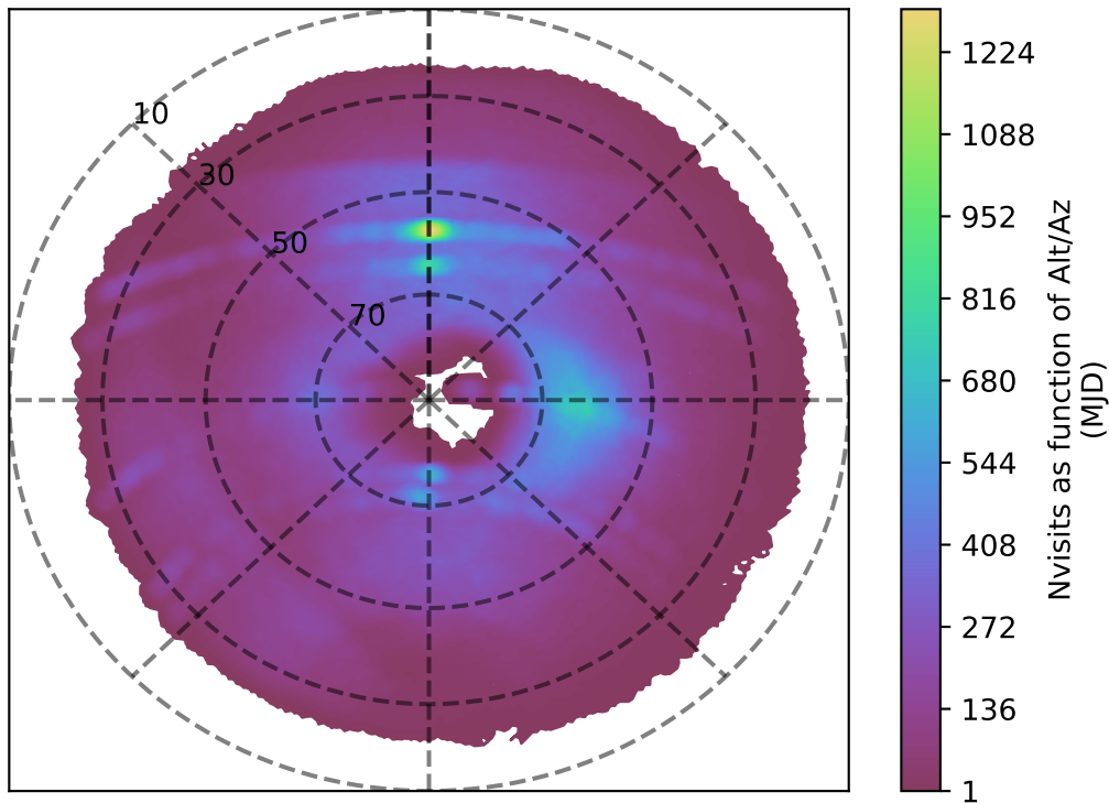
mw_roll_all_v3.3_10yrs g band: Nvisits as function of Alt/Az
