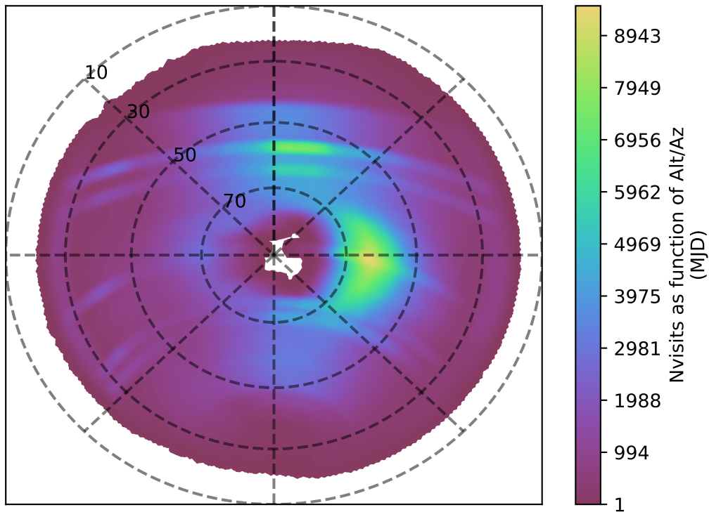
mw_roll_all_v3.3_10yrs all bands: Nvisits as function of Alt/Az
