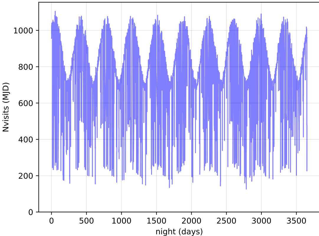
mw_roll_all_v3.3_10yrs All visits: Nvisits
