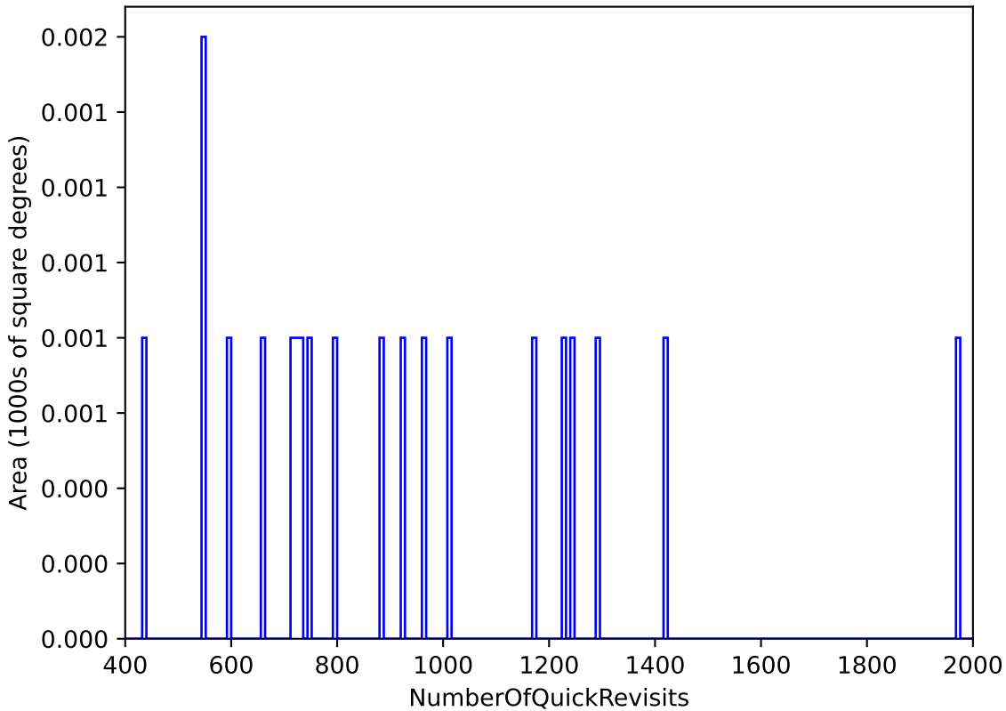
mw_roll_all_v3.3_10yrs WFD: NumberOfQuickRevisits
