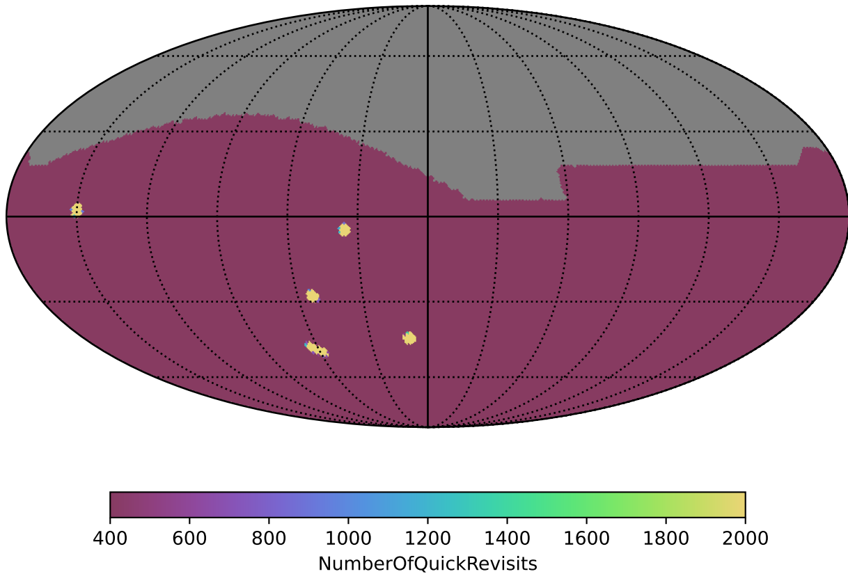
mw_roll_all_v3.3_10yrs All sky: NumberOfQuickRevisits
