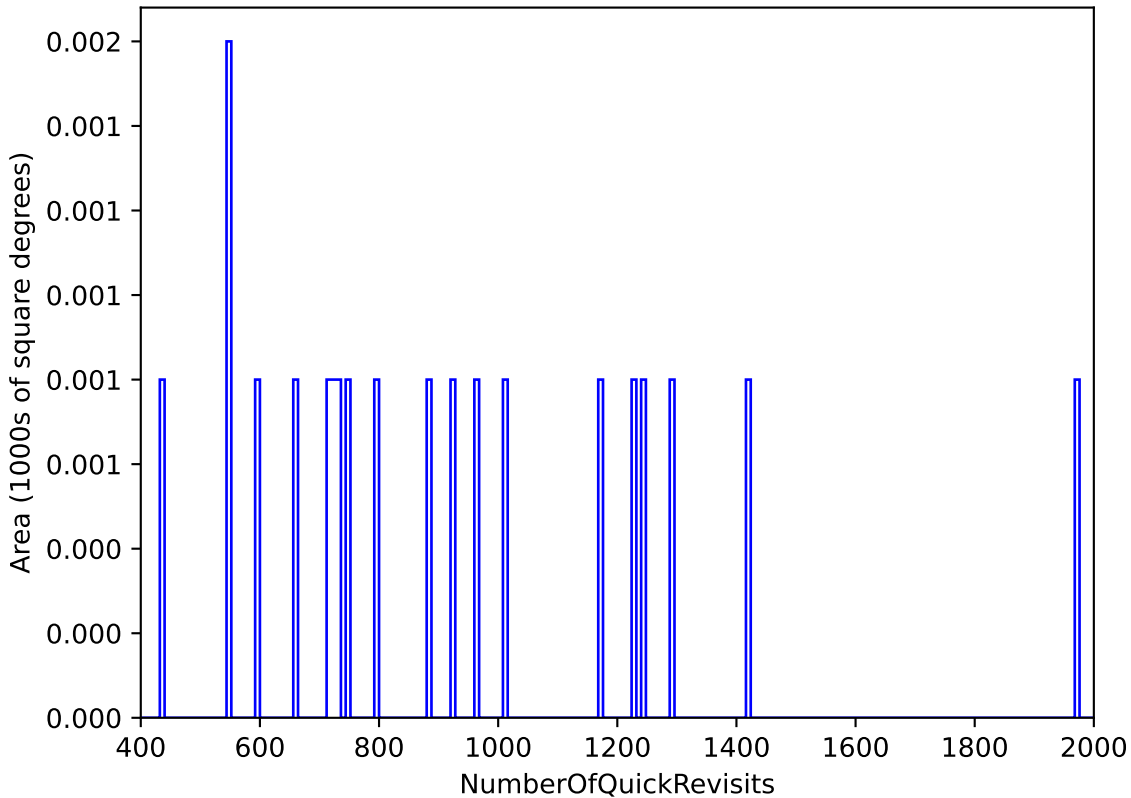
mw_roll_all_v3.3_10yrs All sky: NumberOfQuickRevisits
