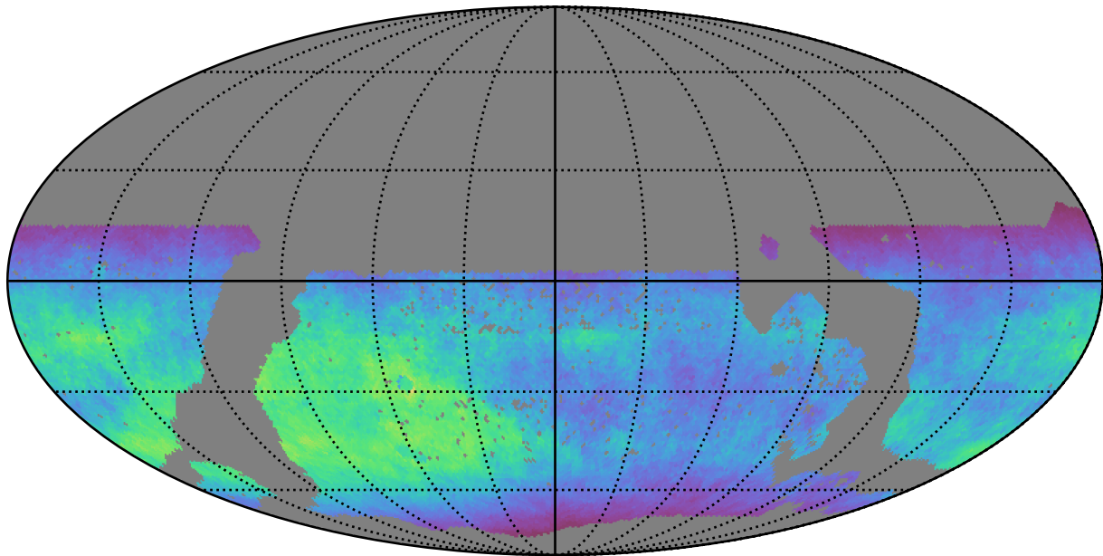
mw_roll_all_v3.3_10yrs WFD z band: Normalized Teff
