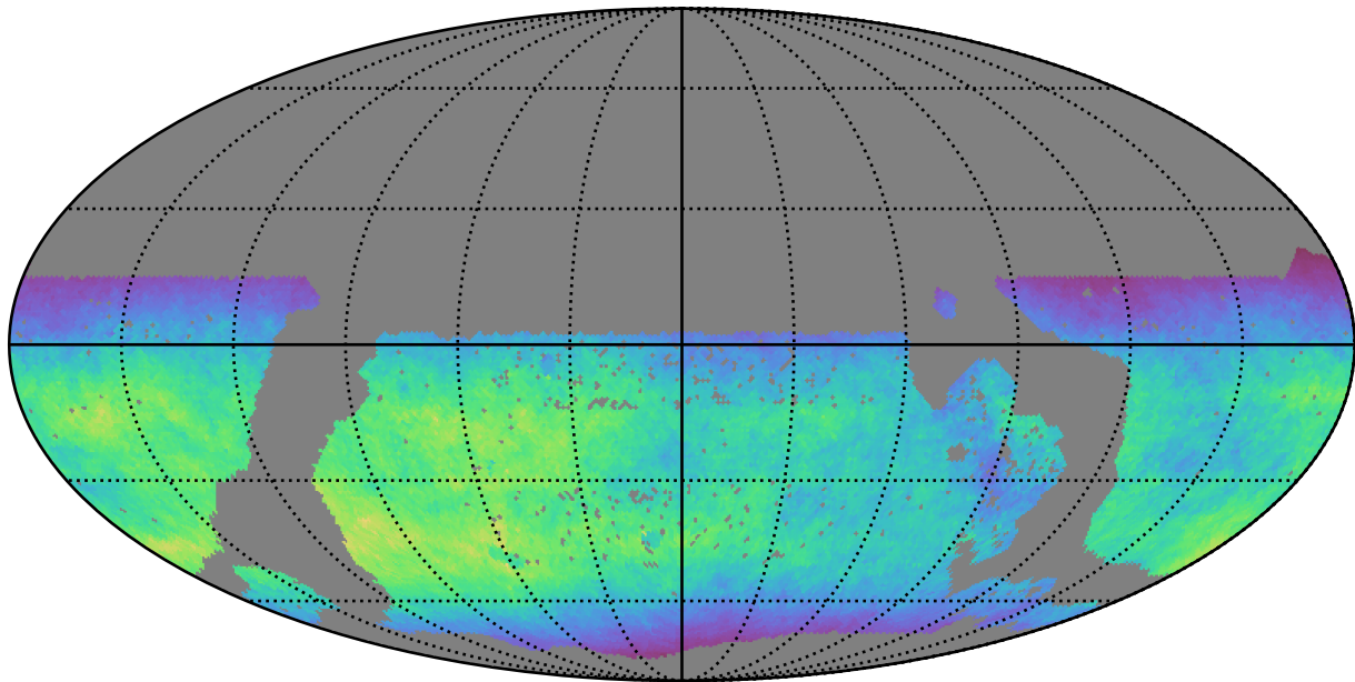
mw_roll_all_v3.3_10yrs WFD y band: Normalized Teff
