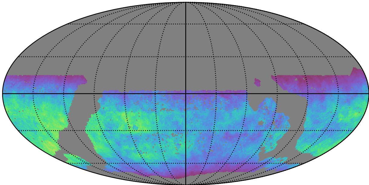
mw_roll_all_v3.3_10yrs WFD u band: Normalized Teff
