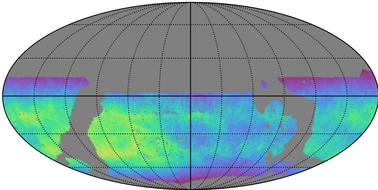
mw_roll_all_v3.3_10yrs WFD i band: Normalized Teff
