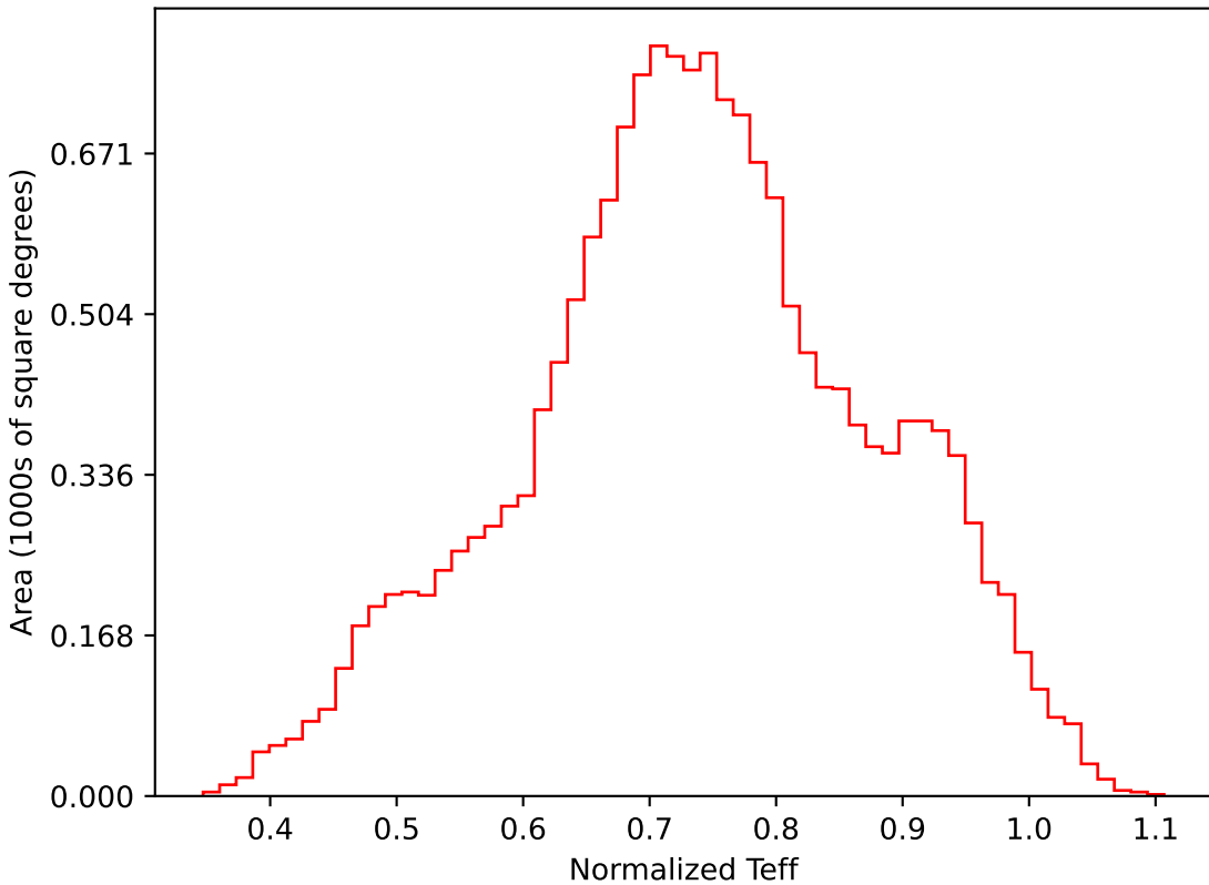
mw_roll_all_v3.3_10yrs WFD i band: Normalized Teff
