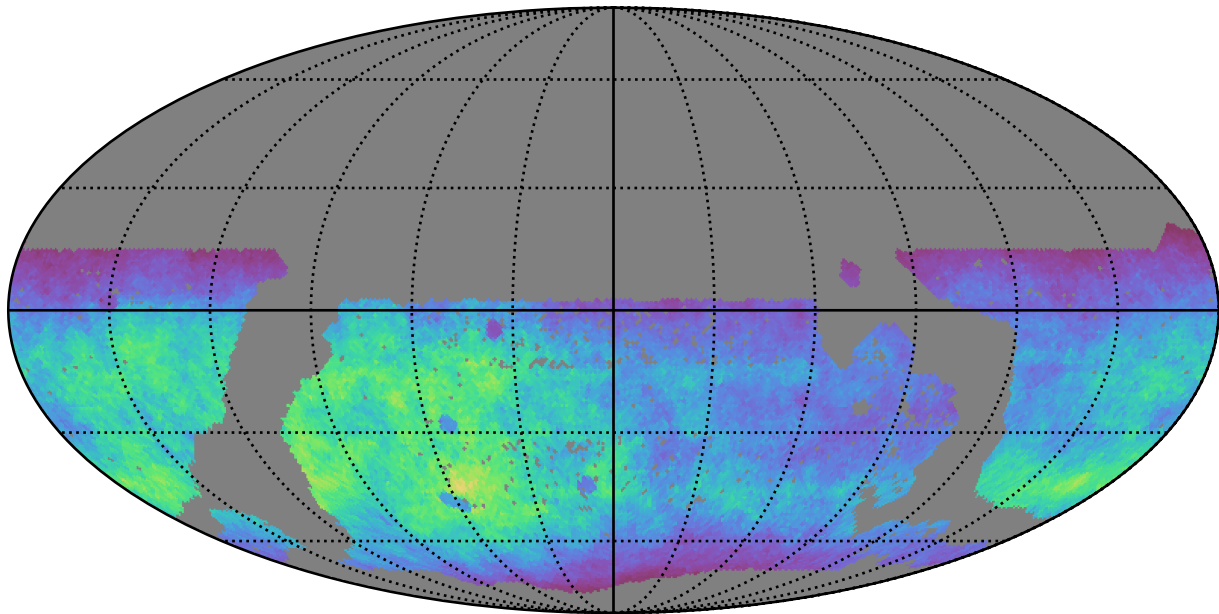
mw_roll_all_v3.3_10yrs WFD g band: Normalized Teff
