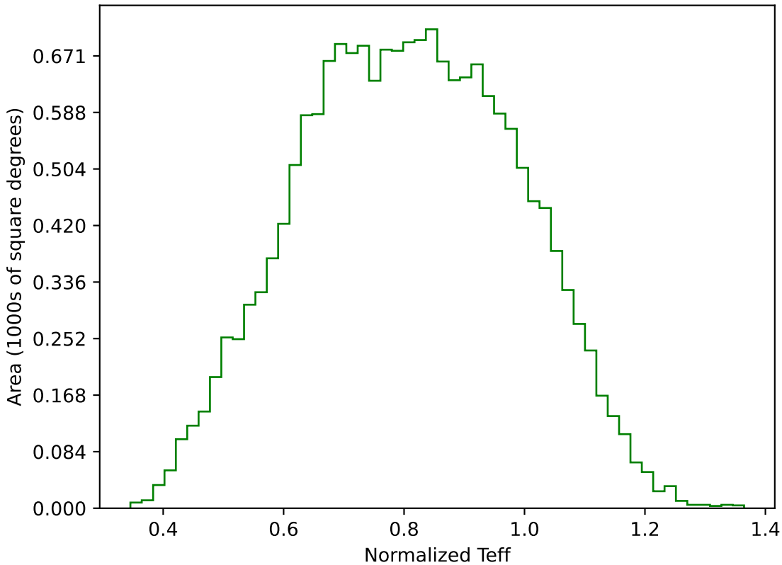
mw_roll_all_v3.3_10yrs WFD g band: Normalized Teff
