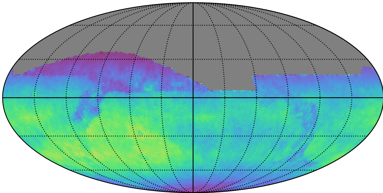
mw_roll_all_v3.3_10yrs All sky z band: Normalized Teff
