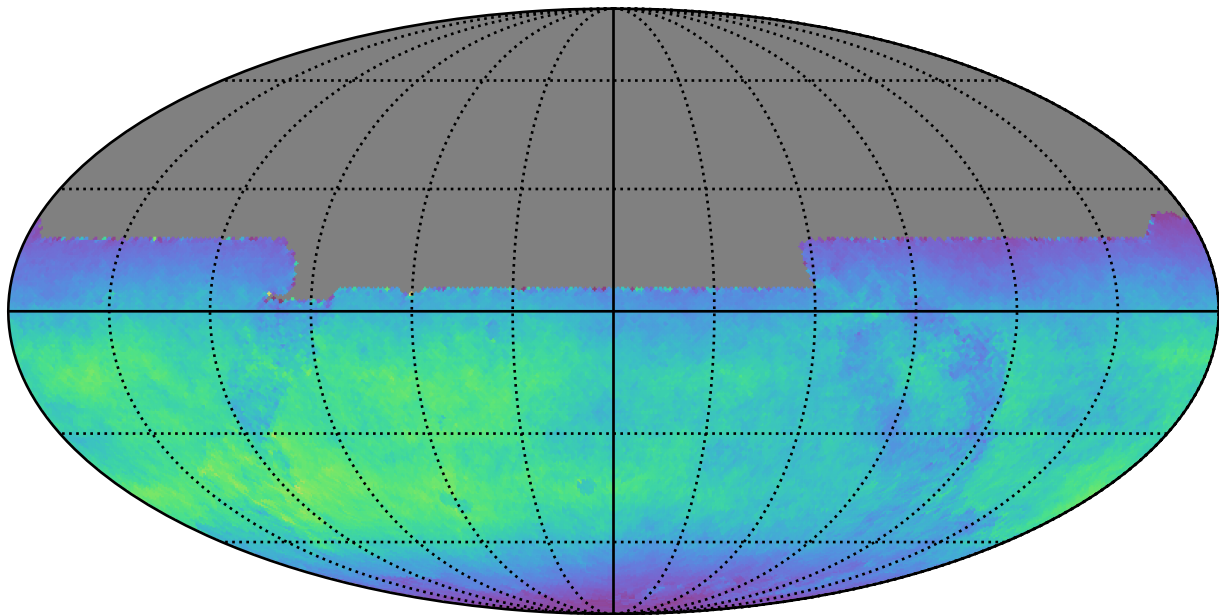
mw_roll_all_v3.3_10yrs All sky y band: Normalized Teff
