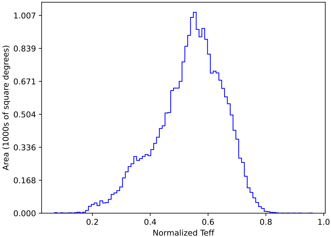
mw_roll_all_v3.3_10yrs All sky y band: Normalized Teff
