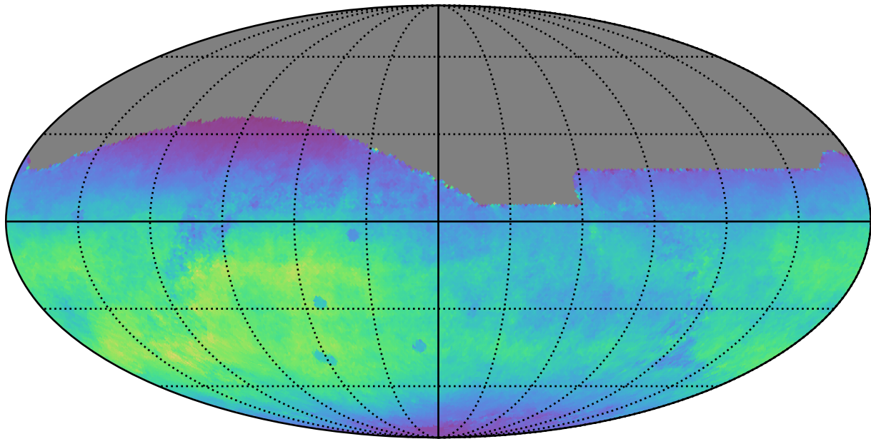
mw_roll_all_v3.3_10yrs All sky r band: Normalized Teff
