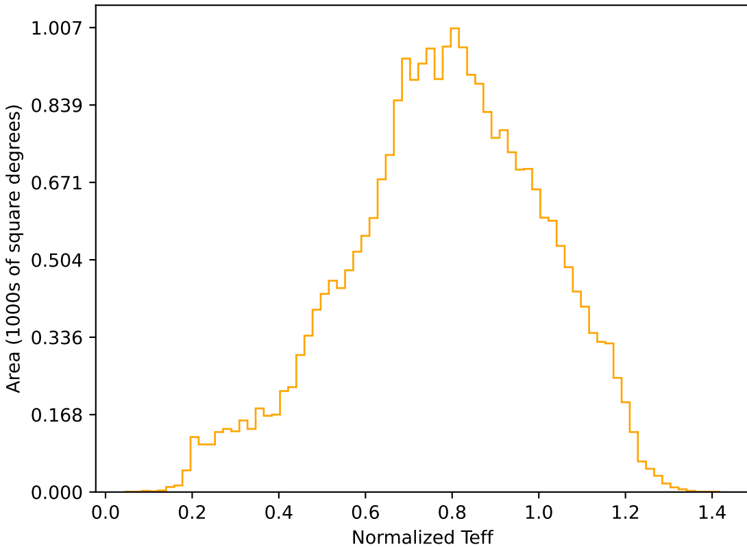
mw_roll_all_v3.3_10yrs All sky r band: Normalized Teff
