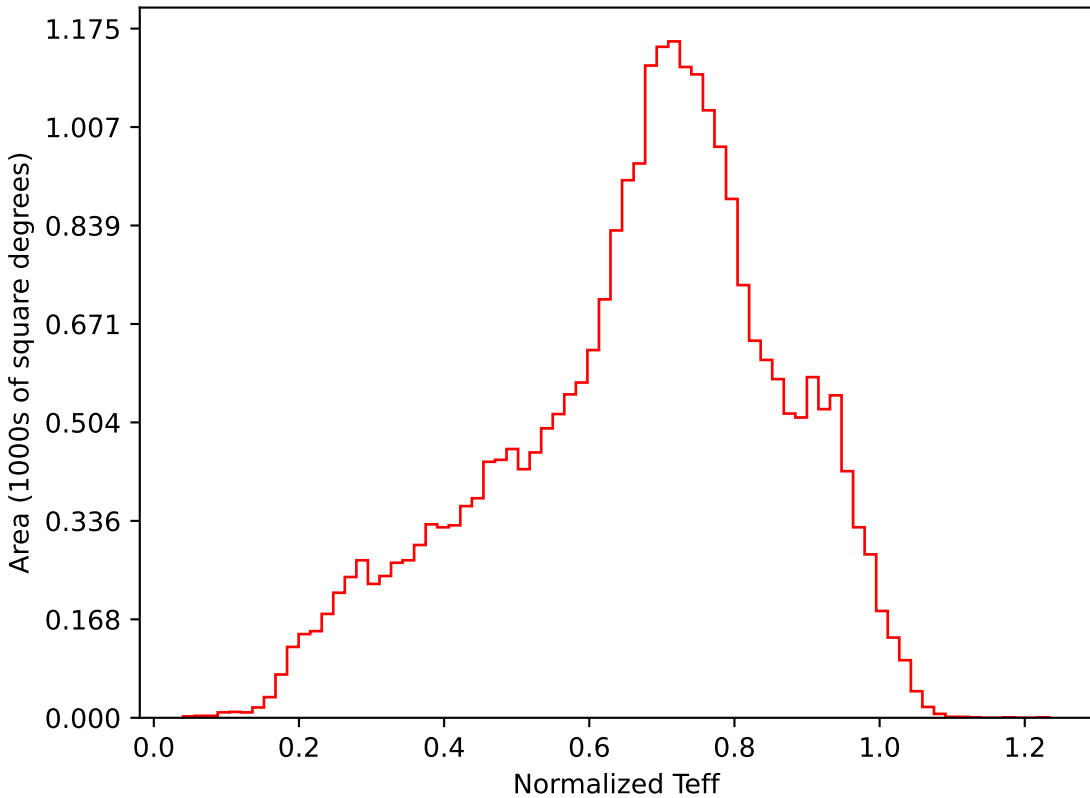
mw_roll_all_v3.3_10yrs All sky i band: Normalized Teff
