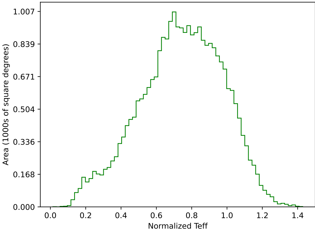
mw_roll_all_v3.3_10yrs All sky g band: Normalized Teff
