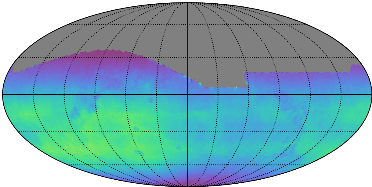
mw_roll_all_v3.3_10yrs All sky all bands: Normalized Teff
