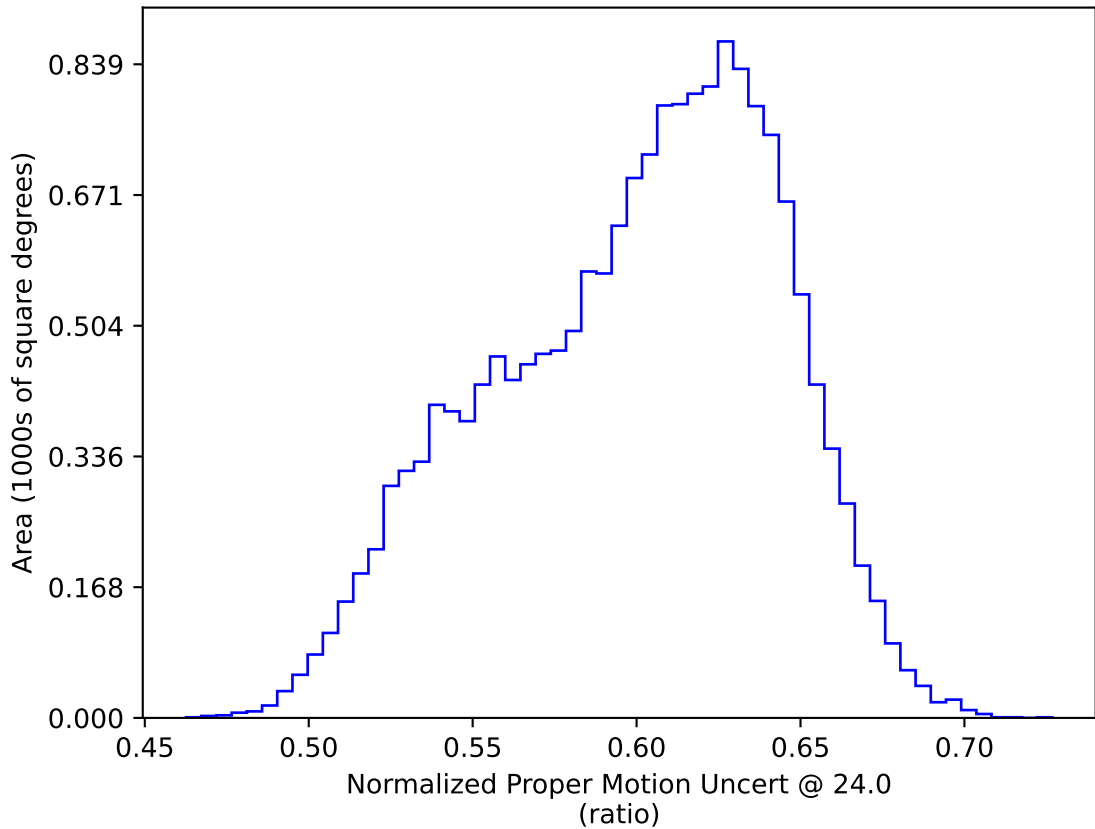
mw_roll_all_v3.3_10yrs WFD: Normalized Proper Motion Uncert @ 24.0
