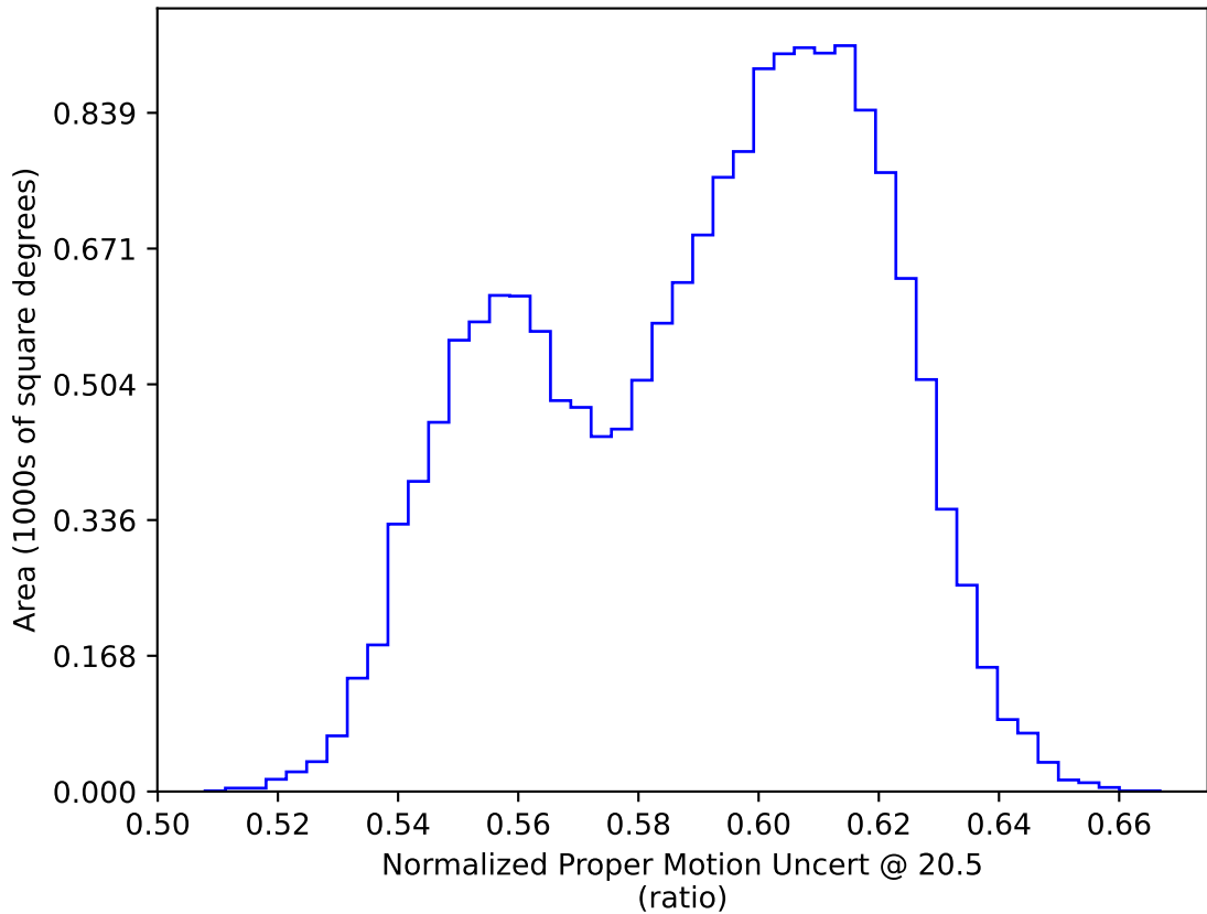
mw_roll_all_v3.3_10yrs WFD: Normalized Proper Motion Uncert @ 20.5
