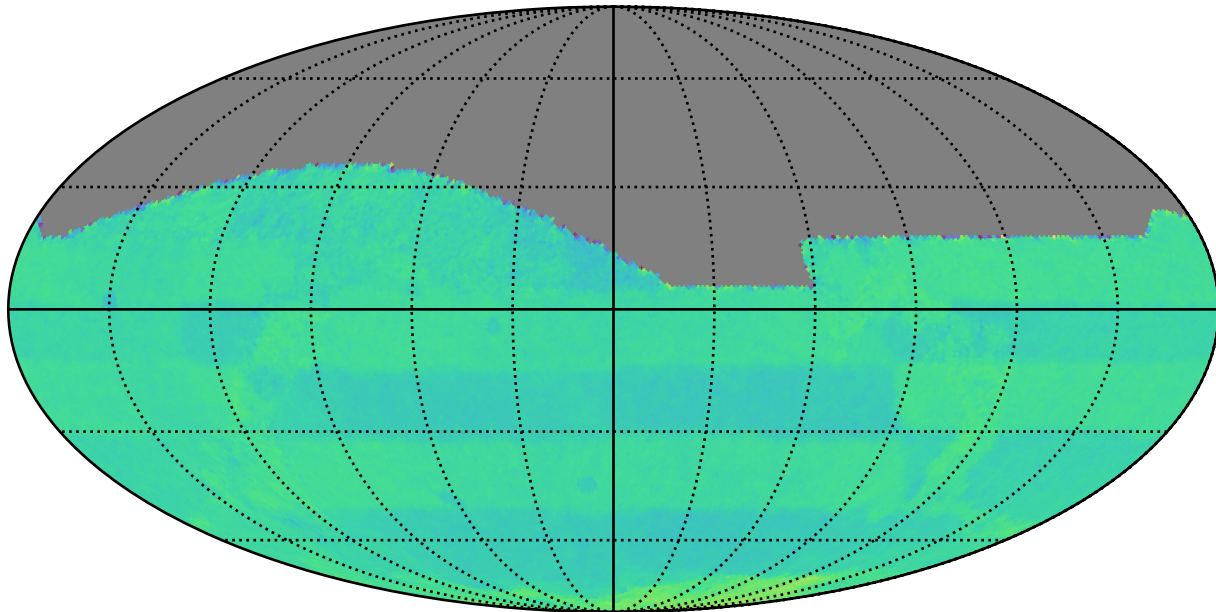
mw_roll_all_v3.3_10yrs All sky: Normalized Proper Motion Uncert @ 20.5
