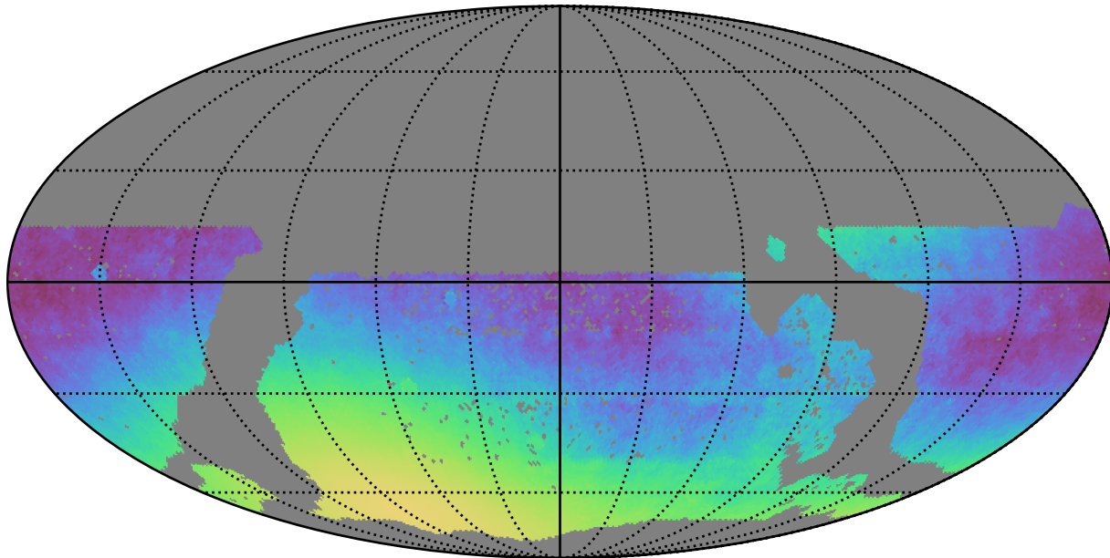
mw_roll_all_v3.3_10yrs WFD: Normalized Parallax Uncert @ 24.0
