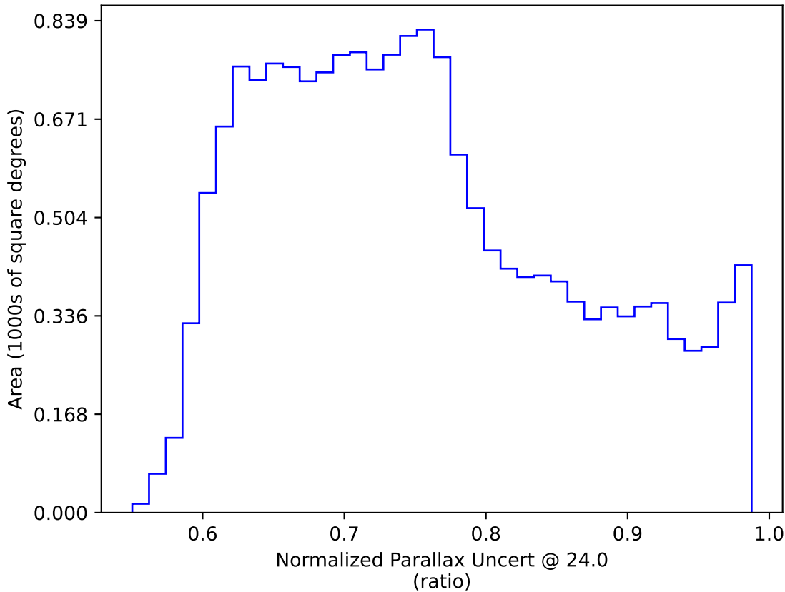
mw_roll_all_v3.3_10yrs WFD: Normalized Parallax Uncert @ 24.0
