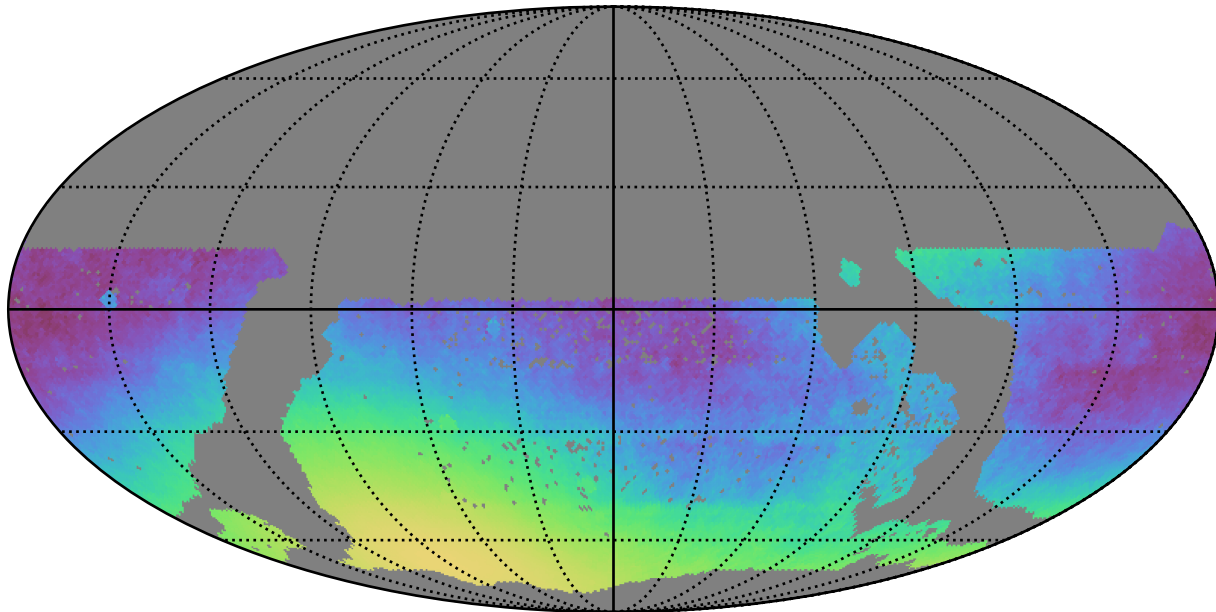
mw_roll_all_v3.3_10yrs WFD: Normalized Parallax Uncert @ 22.4
